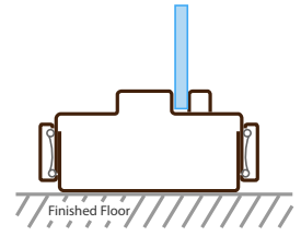
1Q Sill Glazing Flush
