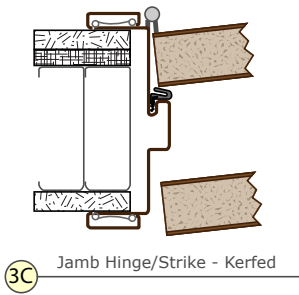
Kerfed Frame - PAIR COMMUNICATING
