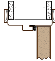
3D Header - Kerfed
