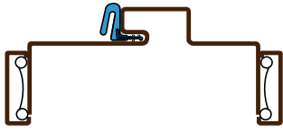
Shown with TA-8 Steel Casing as example.
