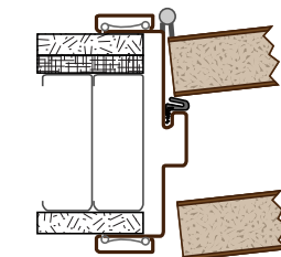
3C Jamb Hinge/Strike - Kerfed
