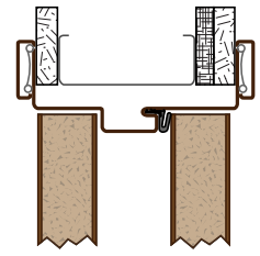
3S Header - Kerfed
